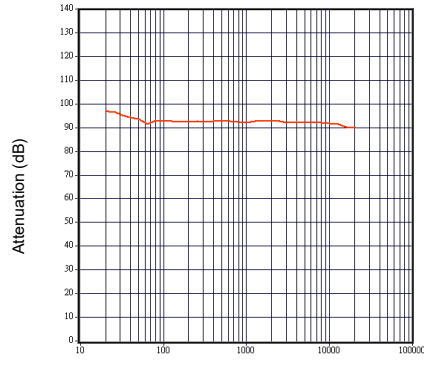
FREQUENCY (Hz) Mute vs. 频率
