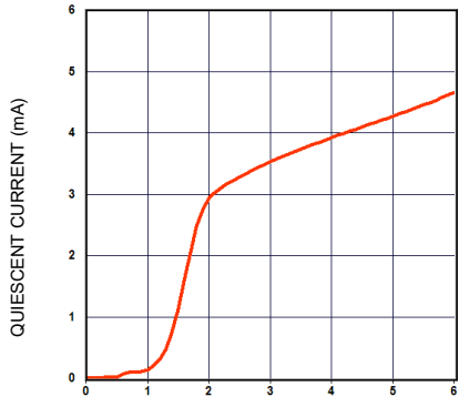
SUPPLY VOLTAGE (V) 靜態電流 VS. 供給電壓
