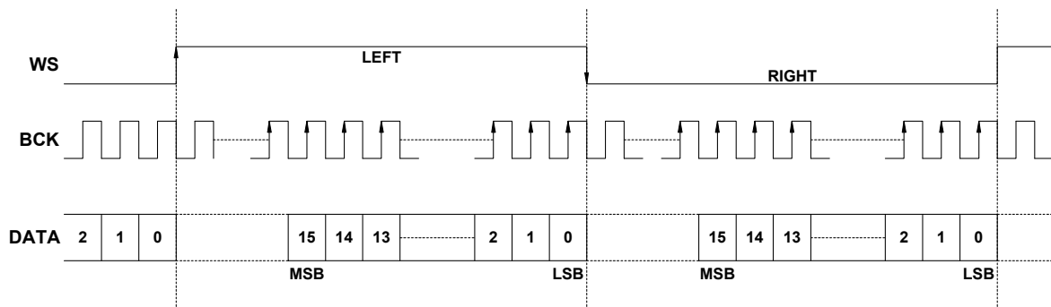
图三、输入信号格式Right justified (MS6326)
