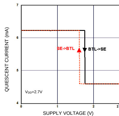
Mode vs. HP-IN votage
