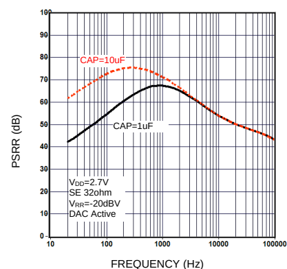
PSRR (2.7V) vs. frequency
