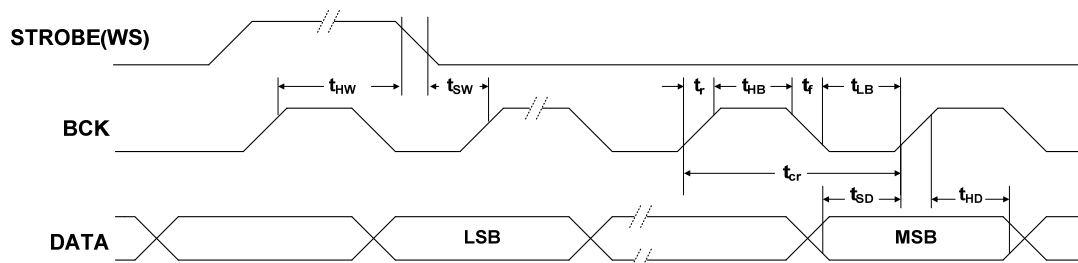
Fig.2 Timing and input signals. (Mono)
