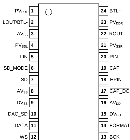
MS6337, SSOP24
