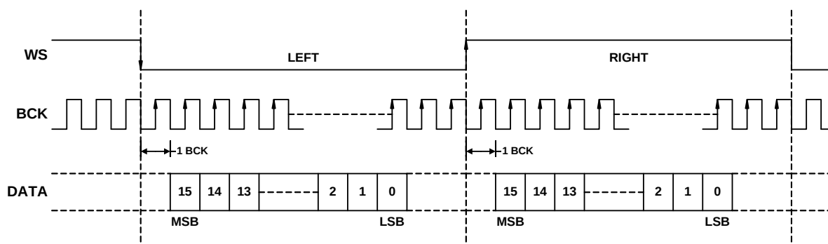
Fig.3 I2S format (Stereo)
