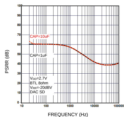
PSRR (2.7V) vs. frequency
