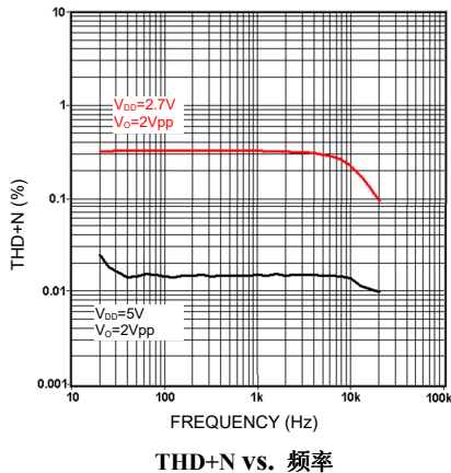
THD+N vs. 频率
