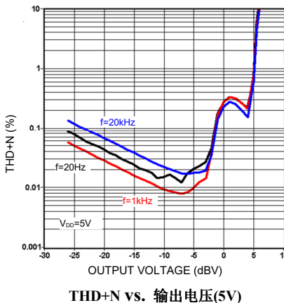
THD+N vs. 输出电压(5V)
