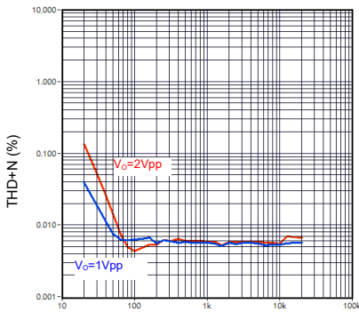
FREQUENCY (Hz) THD+N vs. Frequency
