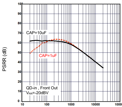
FREQUENCY (Hz) PSRR vs. Frequency
