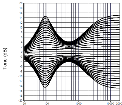
FREQUENCY (Hz) Typical Tone Response
