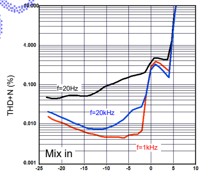
OUTPUT VOLTAGE (dBV) THD+N vs. Output Voltage
