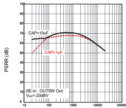
FREQUENCY (Hz) PSRR vs. Frequency
