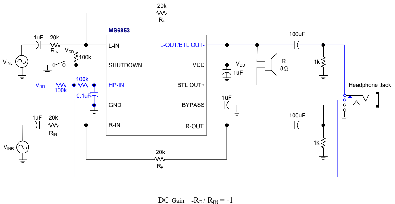
Fig.2 A audio amplifier application circuit. (connected to L-OUT)
